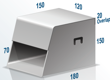
AK2Z BARRIER Z
