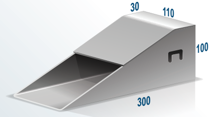
AK6 SHORT TOP LAYBACK
